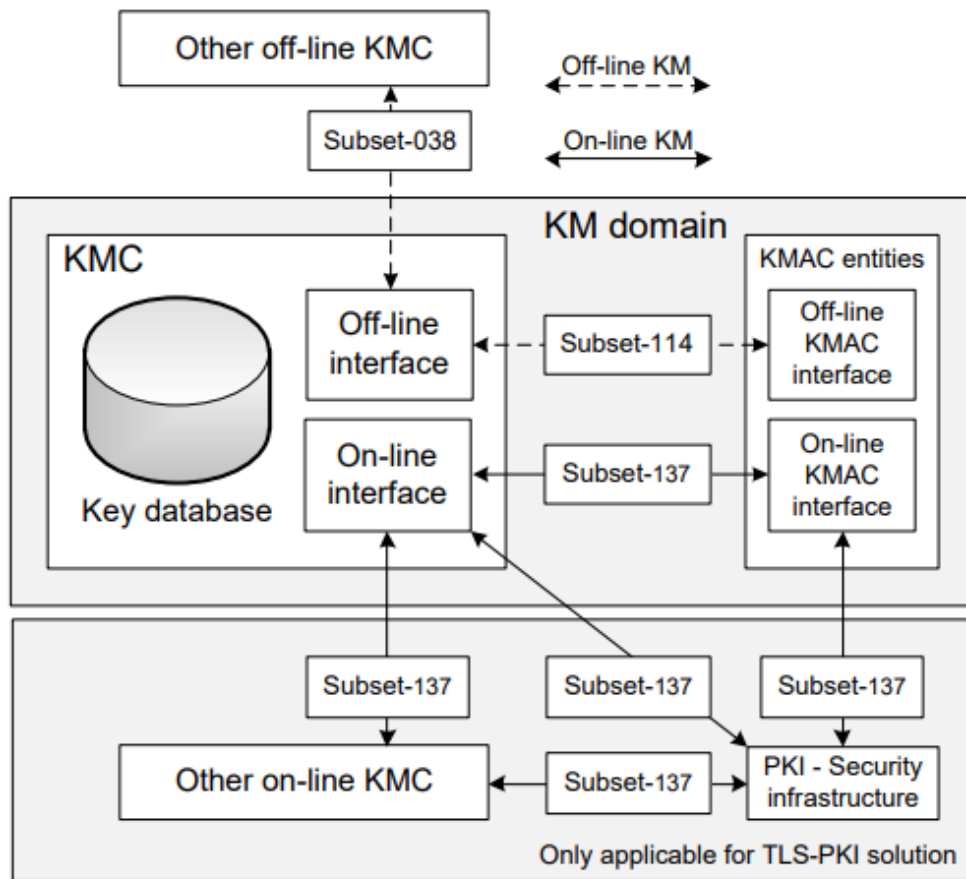
Subset 137 – KMS reference architecture
