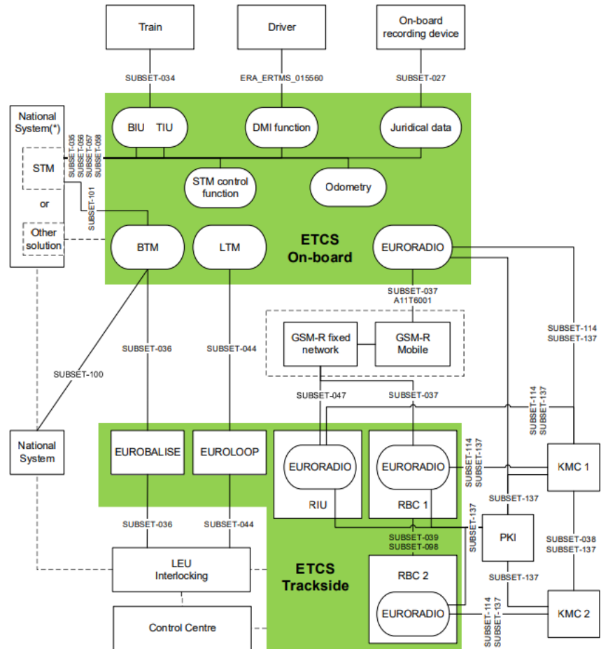
ERTMS/ETCS reference architecture
